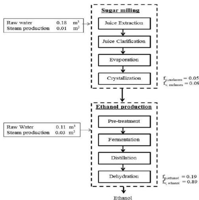
Figure 2. The flowchart of sugarcane-based ethanol production.
