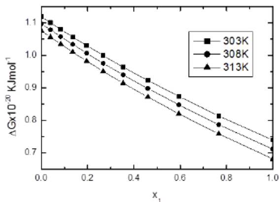
Figure 2. Variation Gibbs free energy with brompheniramin.
