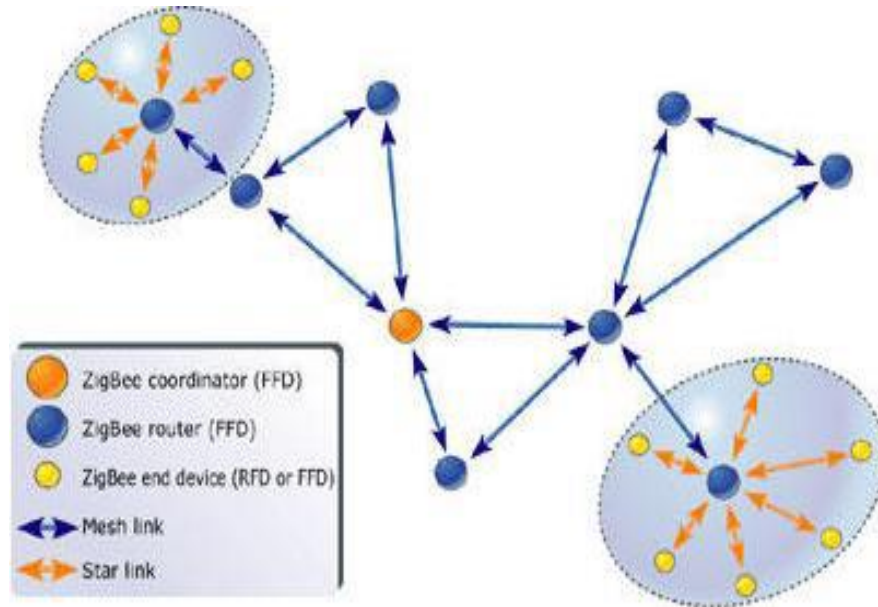
Figure 3: wireless network
