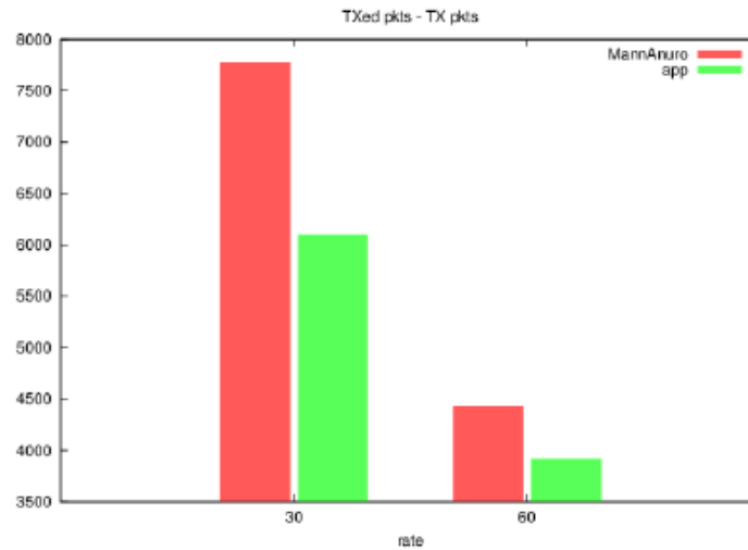
Figure 5. Packets sent by the applications.
