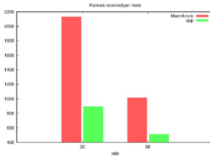
Figure 6. Packets received by applications.
