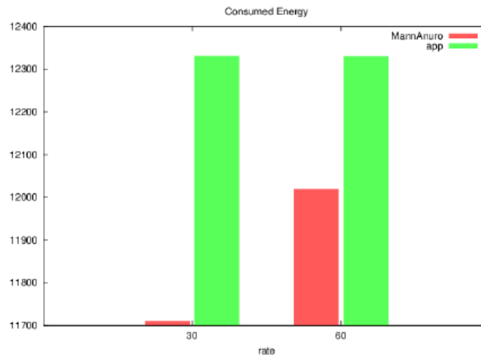
Figure 4. Energy consumed by the sensor nodes.
