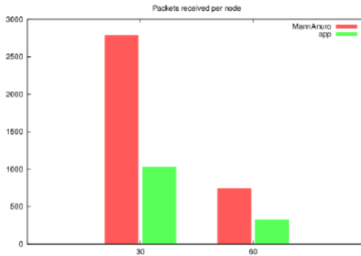
Figure 3. Packets received by applications.
