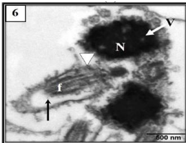
Figure 6: Transmission electron micrographs (TEM) of sperm of polluted L. equulus showing abnormal chromatin content and distribution of most sperm head, sperm exhibiting forked nucleus (N; arrow); neck with absence of mitochondria (arrow head); shortage of the tail and dilation of plasma membrane of the tail (f; black arrow) and vacuoles(V).
