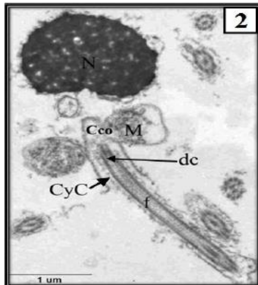
Figure 2: Transmission electron micrograph (TEM) of L. equulus sperm showing cytoplasmic canal (CyC); cytoplasmic collar (Cco); distal centriole (dc); flagellum (f); mitochondria (M) and nucleus (N).
