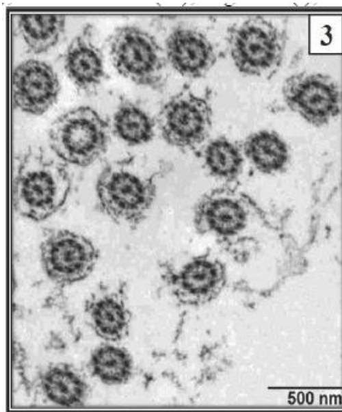
Figure 3: Transmission electron micrograph (TEM) of axoneme of non-polluted L. equulus sperm showing a typical eukaryotic organization, consisting of nine outer doublet microtubules and a central pair of doublet microtubules 9+2 pattern. respect to lateral and longitudinal axis of ovoid nucleus (Fig. 1 & 2). The axoneme showed a typical eukaryotic organization, consisting of nine outer doublet microtubules and a central pair of singlet microtubules 9+2 pattern (Fig. 3).
