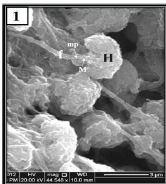
Figure 1: Scanning electron micrograph (SEM) of the spermatozoon of L. equulus showing flagellum (f); head (H); mid piece (mp) and mitochondria (M).
