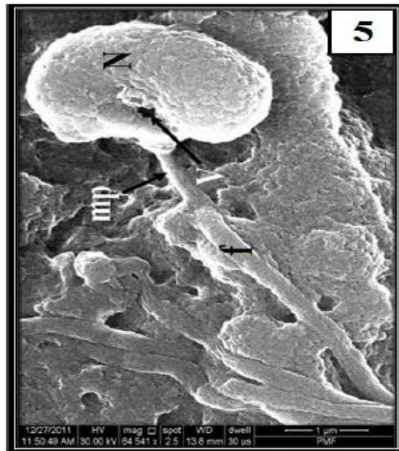
Figure 5: Scanning electron micrograph (SEM) of sperm of polluted L. equulus showing abnormal granulated chromatin sperm head having vacuoles (V) and absence of mitochondria; flagellum (f); mid piece (mp) and nucleus (N).
