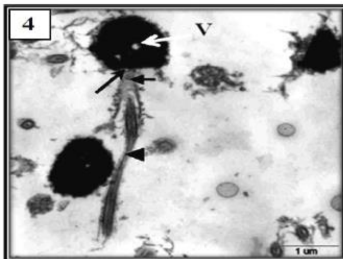
Figure 4: Transmission electron micrographs (TEM) of sperm of polluted L. equulus showing abnormal spermatozoa having elliptical head, absence of mitochondria (short arrow); adhesion of sperm head to cytoplasmic collar (long arrow); the middle piece is completely absent and axonemal defect (arrow head) and vacuole (V).
