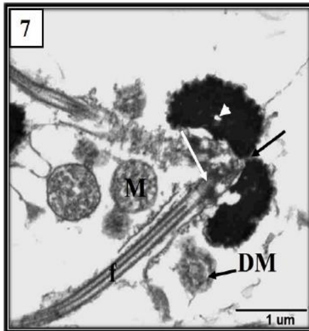
Figure 7: Transmission electron micrographs (TEM) of sperm of polluted L. equulus showing abnormal sperm with head-to-head agglutination (black arrow); degenerated mid piece separating from sperm head (white arrow); distorted mitochondria (DM); flagellum (f) and mitochondria (M).
