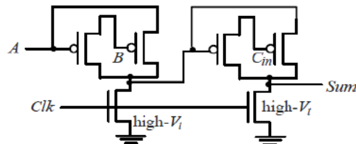
Fig 2. SUM Circuit
