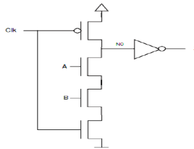
Fig.4: 2 input AND Gate using Domino Logic
