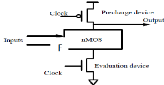
Fig.1 Basic structure of Domino Logic
