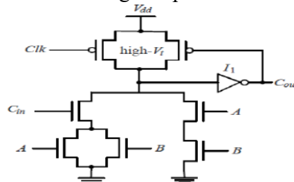
Fig.3: CARRYOUT Circuit
