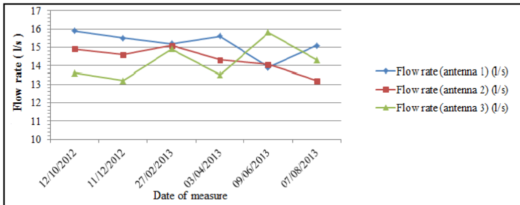
Figure 4- Mean flow rate of the irrigation antennas during the agricultural year (2012/2013)
