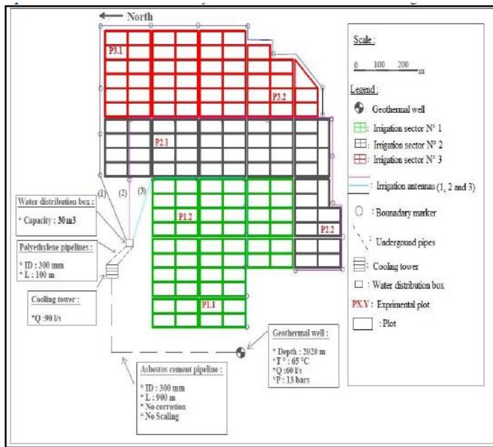
Figure 2- Land plot plan of Lazala oasis and the hydraulic network
