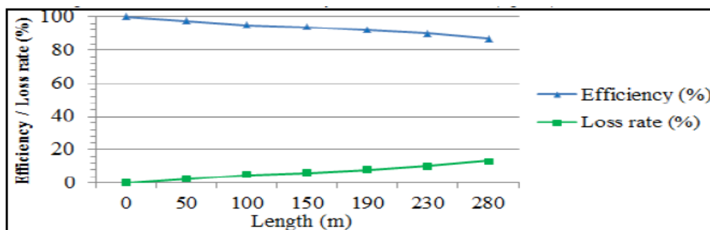
Figure 6- Spatial evolution of the losses and the efficiencies of the tertiary irrigation network
