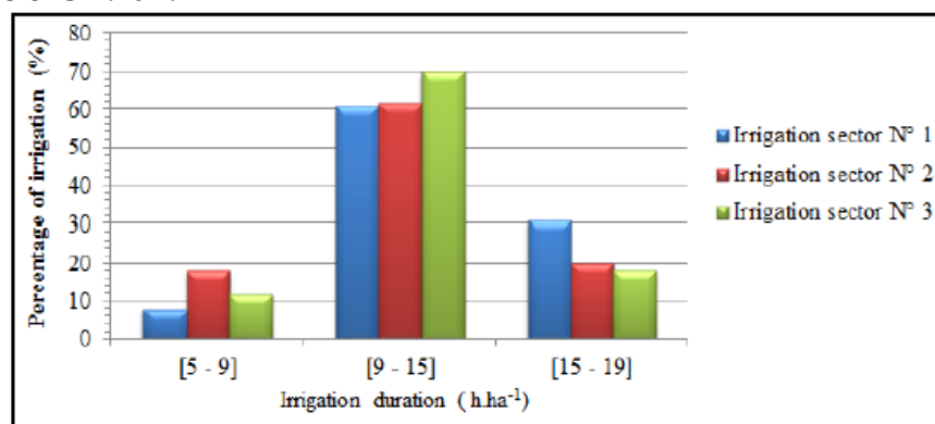
Figure 8- Histogram of irrigation duration with respect to current rule of 9h.ha -1 (number of irrigated plots: 150, number of irrigation events: 1429, agricultural year 2012/2013).
