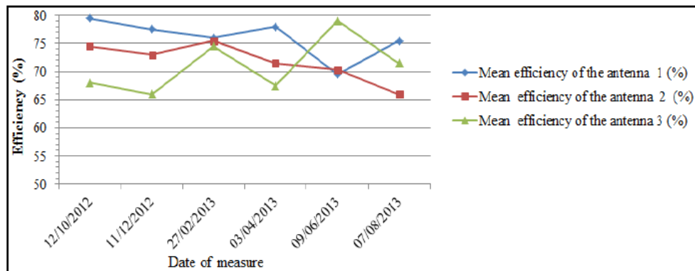
Figure 5- Temporal evolution of the mean efficiencies for the irrigation antennas
