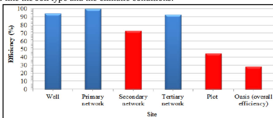
Figure 9- Irrigation performance from the well to the plot during the study year
