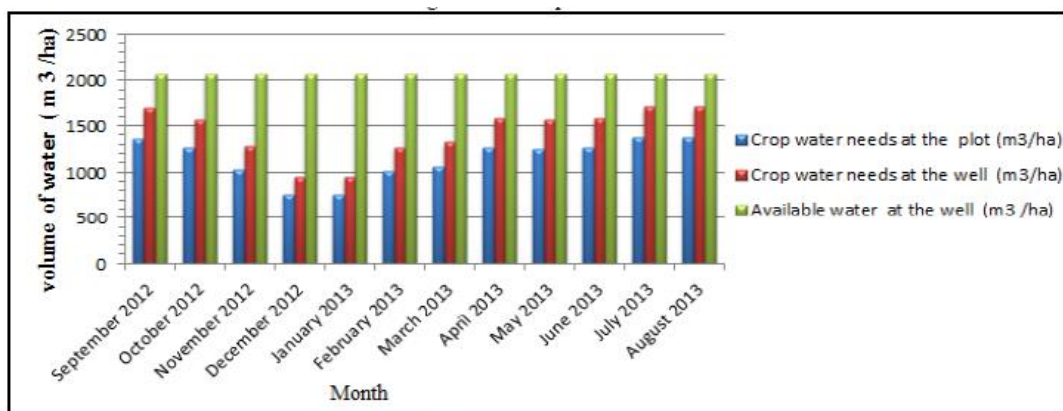
Figure 3- Availability of irrigation water and crop water requirements
