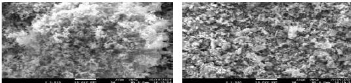
Fig-3(a): SEM image of ZnO dried at 140°C Fig-3(b) SEM image of ZnO dried at 180°C
