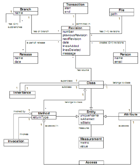
Figure 2: Historical analysis for source code with EVOLIZER data schema.
