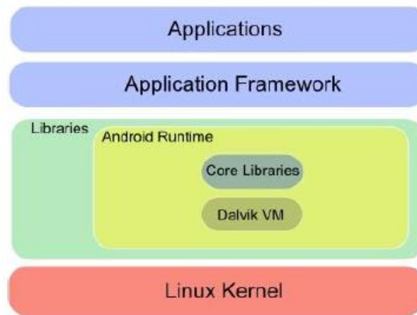
Figure (3) Android platform components. [2]
