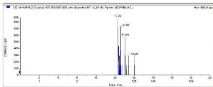
Fig. 9: The LC-MS/MS MRM chromatogram of fipronil and its metabolites. RT:10.29 – Fipronildesulfinyl; RT: 10.57 – Fipronil; RT: 11.04 – Fipronil sulfide; RT:12.05 – Fipronil sulfone
