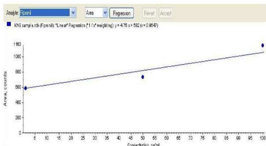
Fig 8: Calibration curve of Fipronil
